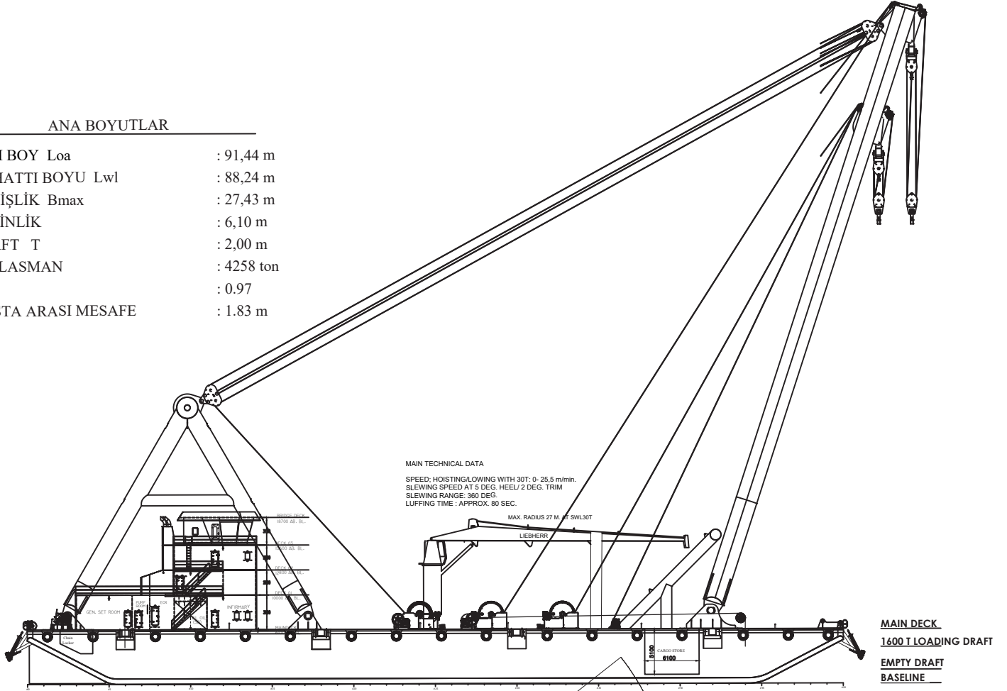
PROFILE VIEW
